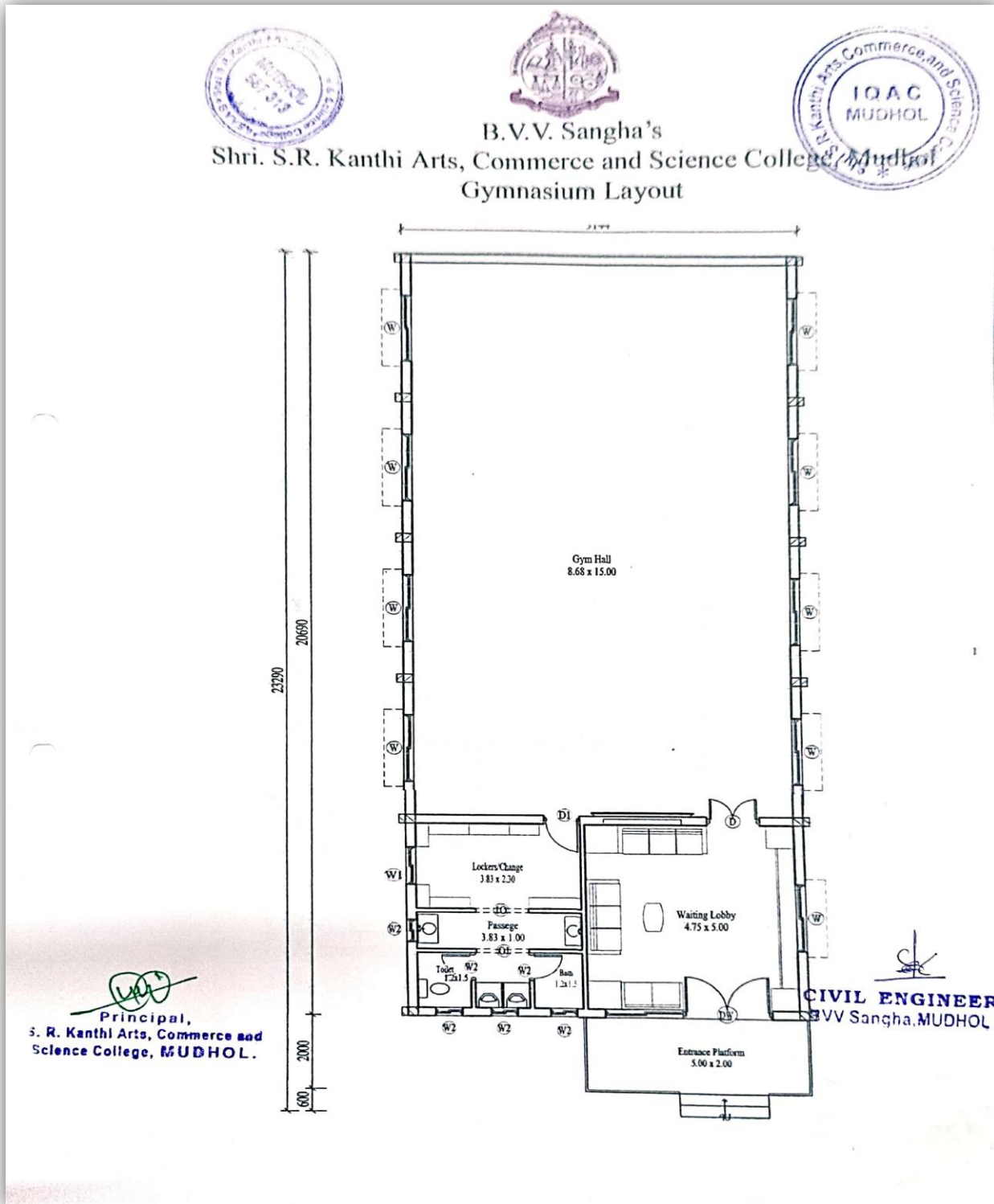
MULTIGYM LAYOUT
