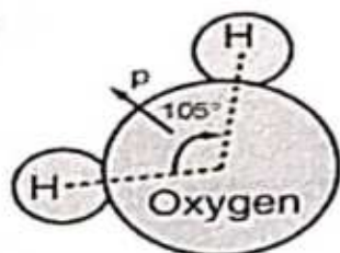
Water molecule with symmetry axis
