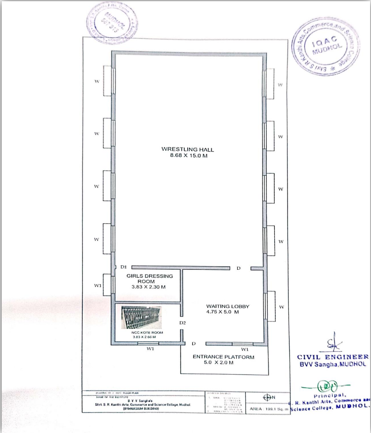
WRESTELLING HALL LAYOUT
