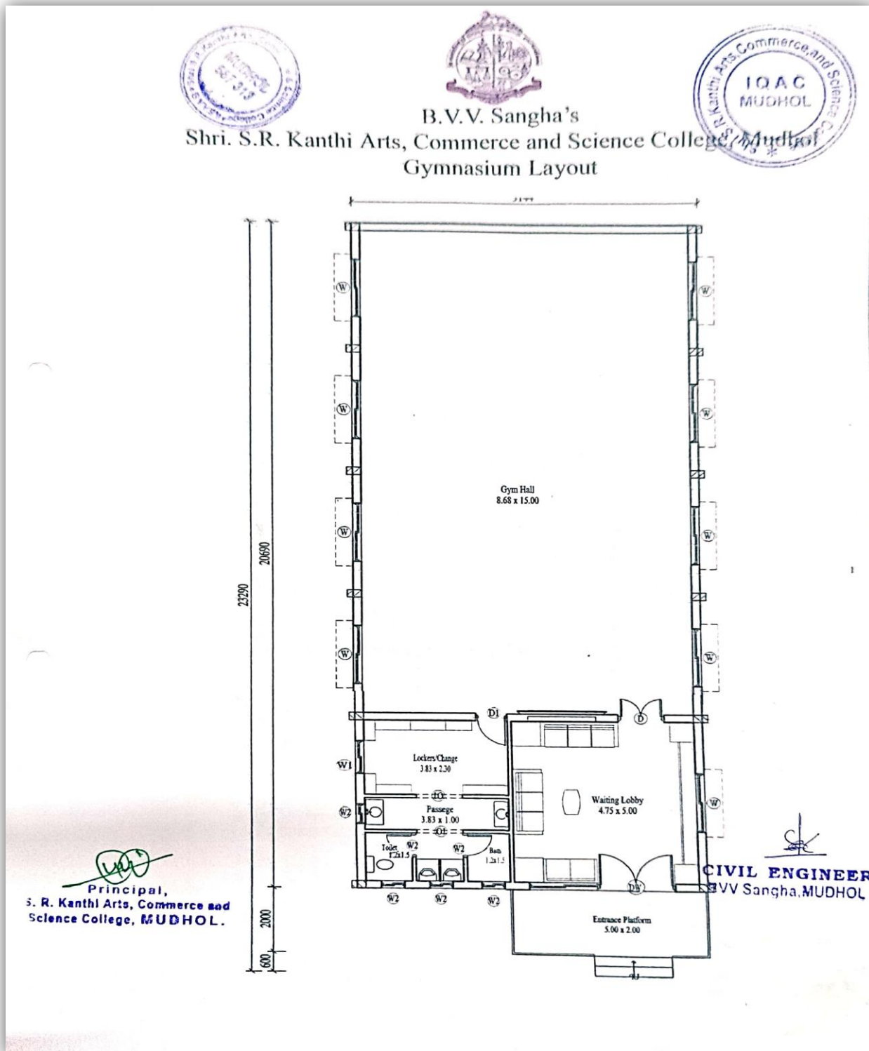
MULTIGYM LAYOUT
